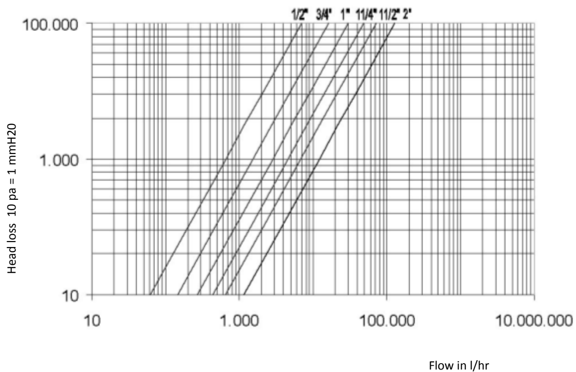
HEAD LOSS DIAGRAM
