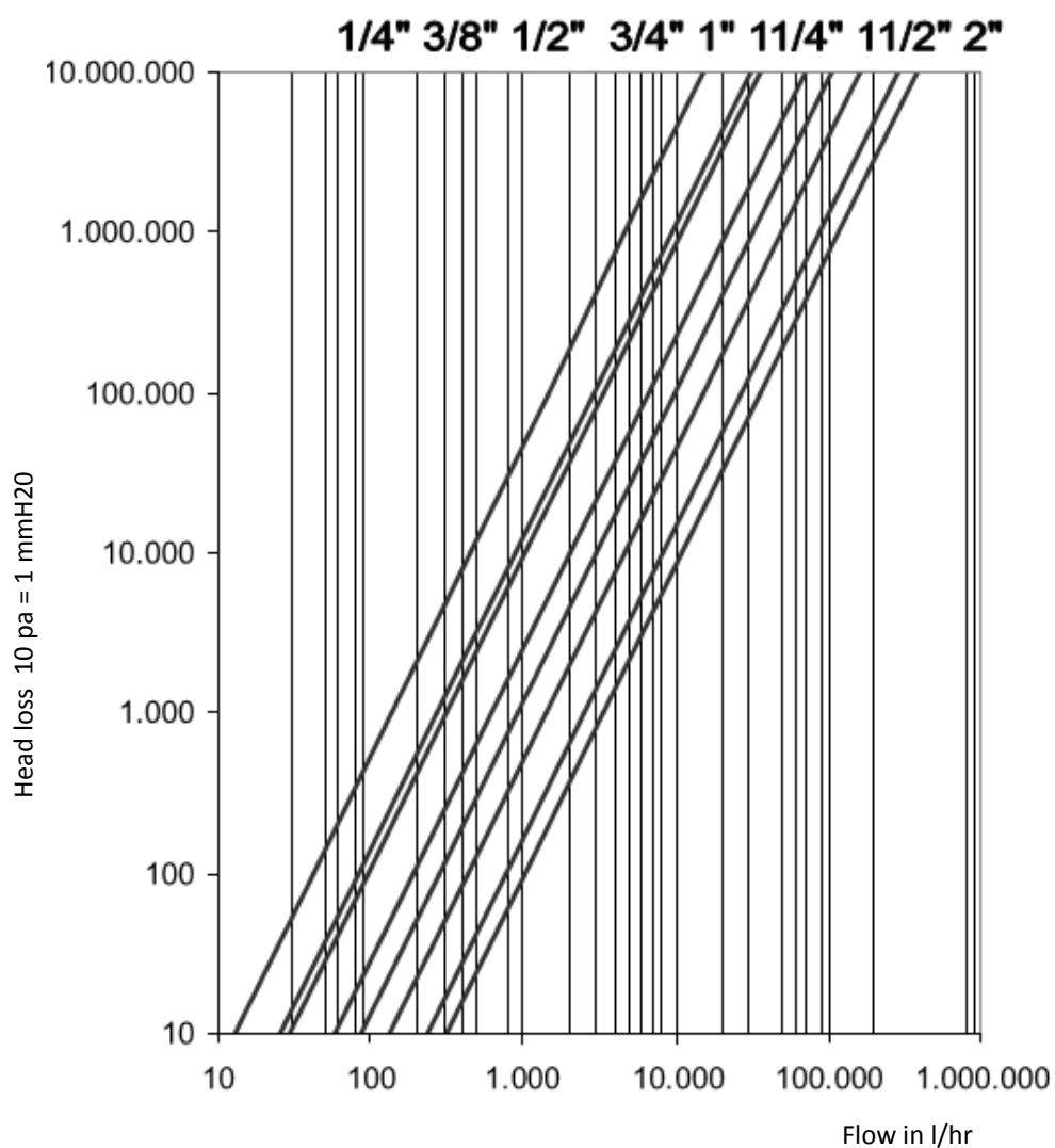
HEAD LOSS DIAGRAM
